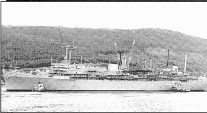
Largest in displacement was the 20,500-ton submarine tender USS Hunley (AS-31) built at Newport News in 1961 and modified in 1973/1974 to support the Poseidon missile program. Sistership Holland (AS-32) was built by Ingalls a year later. This 1962 photo shows Hunley as built with a large gantry crane for missile loading located well aft. Inset photo shows the much-altered Hunley at Holy Loch circa 1990 being pushed into her mooring by the harbor tugs Piqua and Natick .
